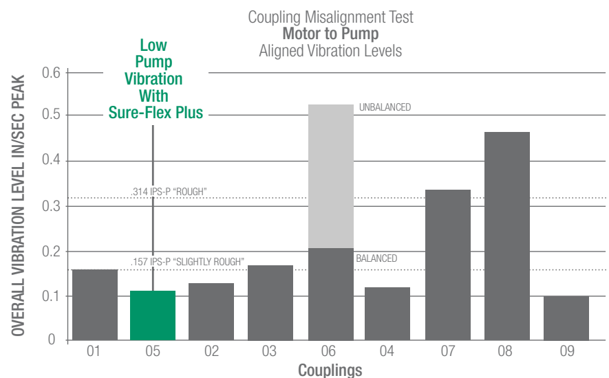
Figure 1: Aligned Pump Overall Vibration Levels with Different Couplings Installed.*
