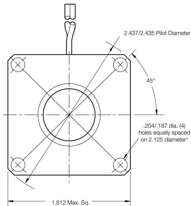
Magnet View
