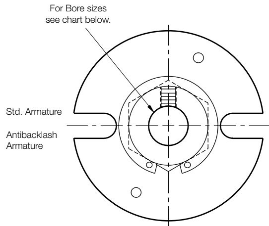
Armature View
