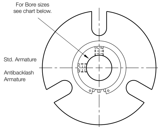
Armature View
