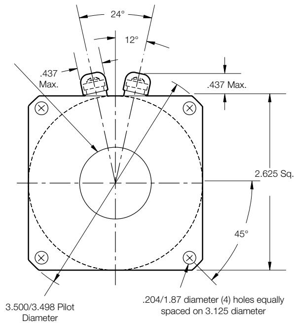
Field View
