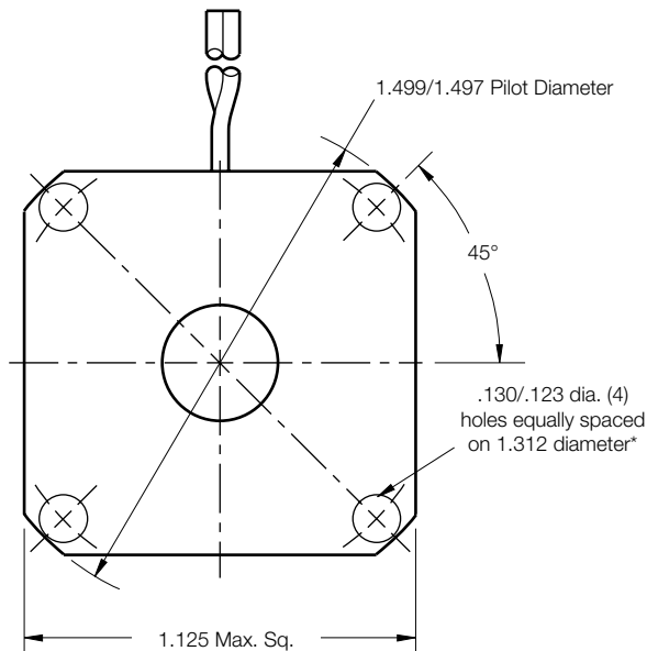
Magnet View
