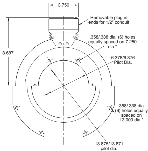
Magnet View (Inside & Outside Mounted)
