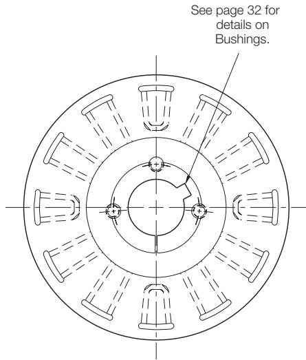
Armature View
