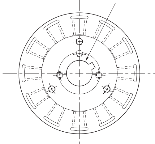
Armature View
