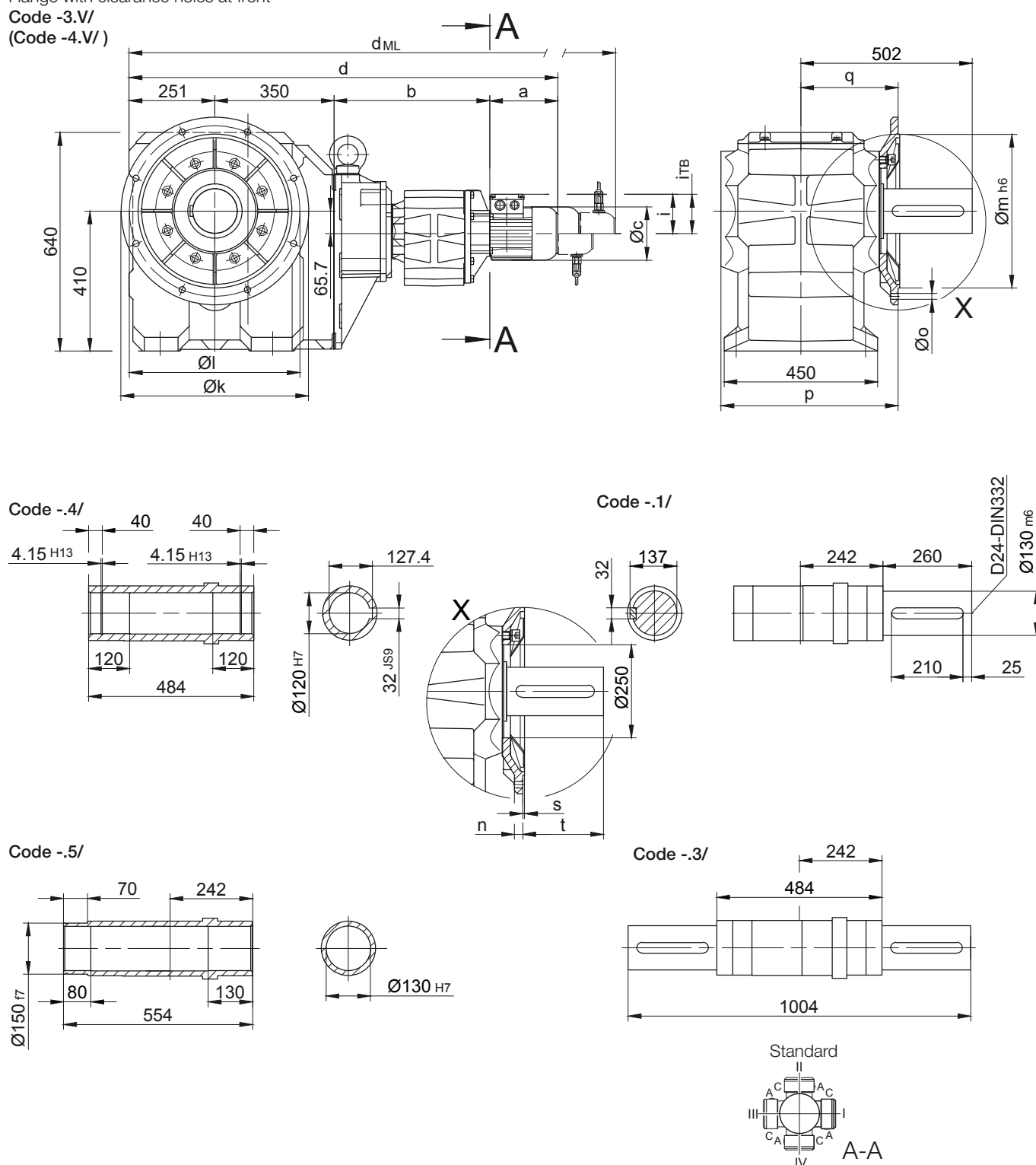
Flange Dimensions
