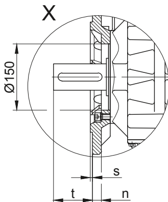
Flange Dimensions
