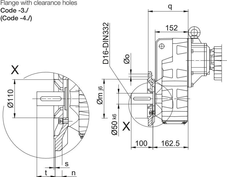
Flange Dimensions
