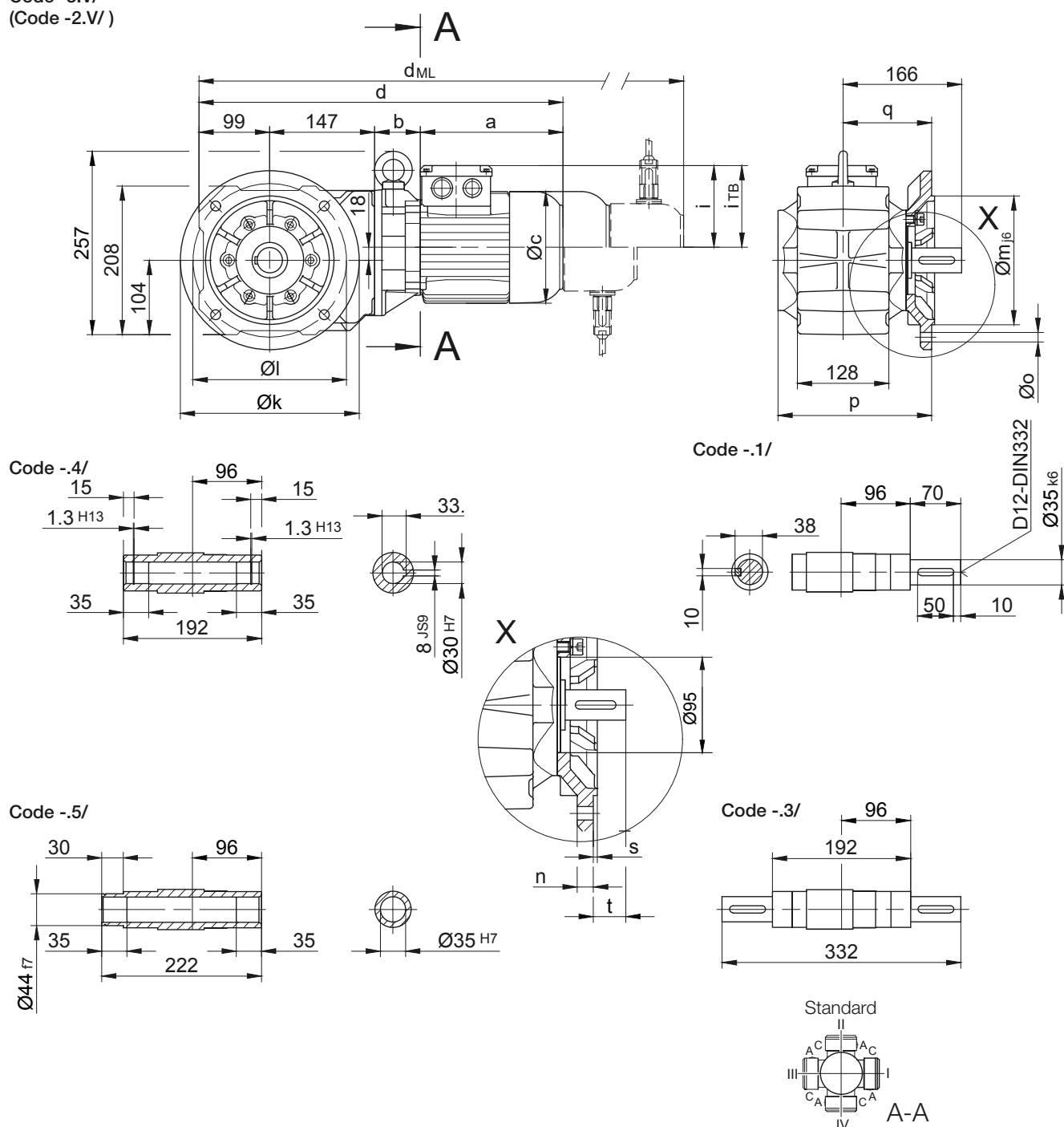
Flange Dimensions
