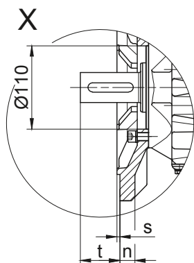
Flange Dimensions
