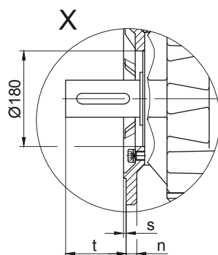
Flange Dimensions
