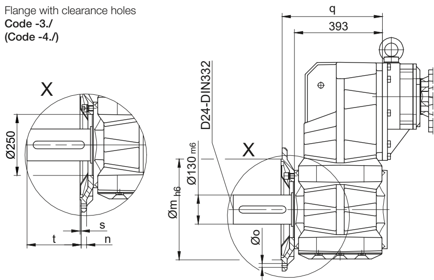
Flange Dimensions
