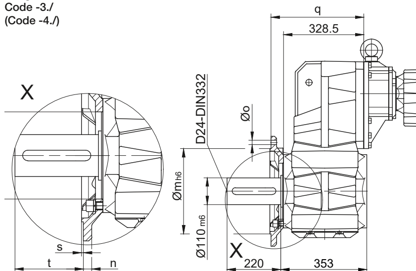
Flange Dimensions
