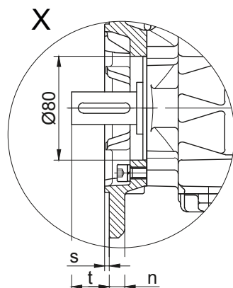
Flange Dimensions
