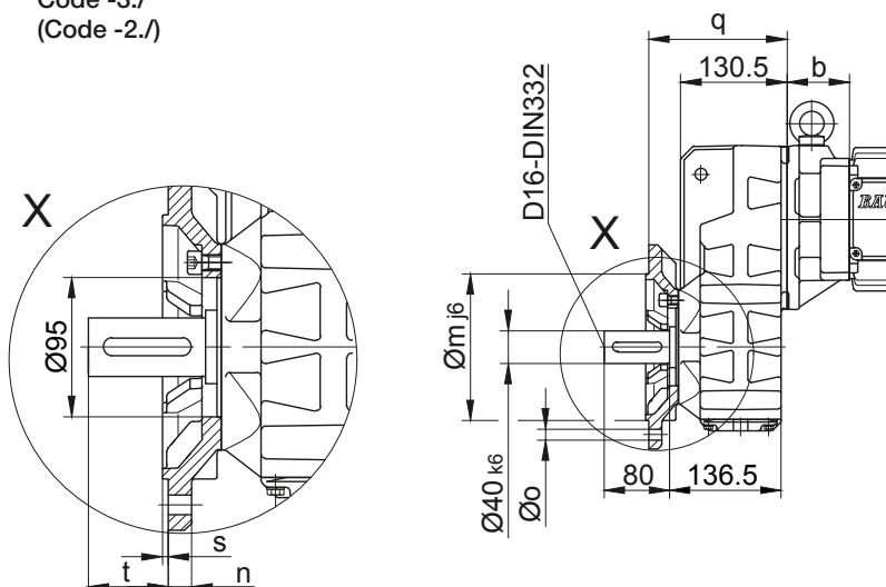
Flange Dimensions
