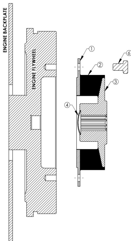
FIGURE 1.1 NV COUPLING CROSS SECTION
