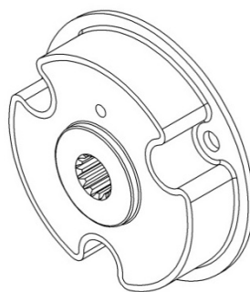
FIGURE 1.4 NV K135 COUPLING (PUMP SIDE)
