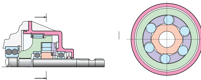
Overrunning clutch for two directions of rotation, automatic change of direction
