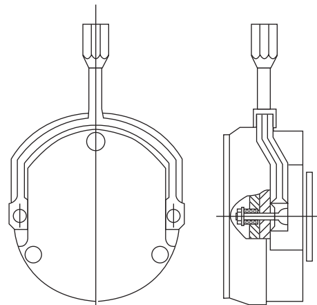
VAR 02 • Torque reduction up to 50% by loosening one nut. • Available in all sizes. • Central nut has several "Detents" per turn allowing accurate torque adjustment. • The brake is factory set at the minimum torque (50% of max. torque).
