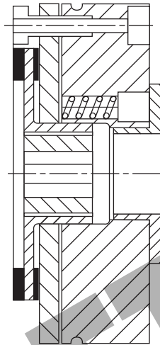
VAR 02 • Torque reduction up to 50% by loosening one nut. • Available in all sizes. • Central nut has several "Detents" per turn allowing accurate torque adjustment. • The brake is factory set at the minimum torque (50% of max. torque).
