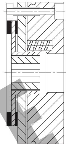
VAR 00 No torque adjustment possible • Available in all sizes. • No hand release option available.
