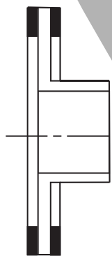
Available in two styles M – Metallic (Standard) S – Thermoplastic (Low inertia) Sizes 005 & 010 only • Large thermoplastic bore hubs (Available in sizes 005 and 010 only) • Large bore metallic disc (Available in sizes 005 thru 035) • High torque metallic discs (Available in sizes 060 thru 300. Requires lower speed of rotation.)
