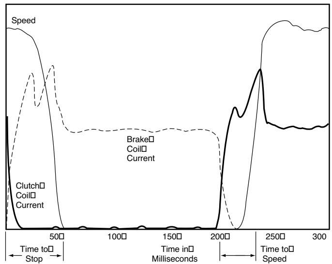
Chart 2 With Overexcitation
