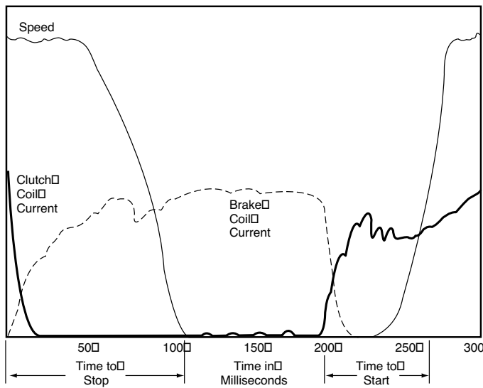
Chart 1 Without Overexcitation
