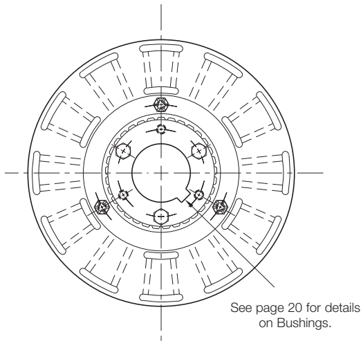
Armature View
