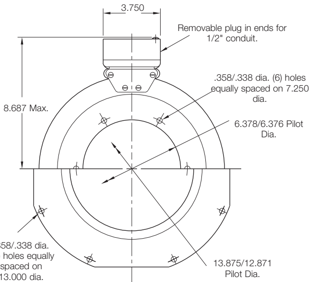
Magnet View
