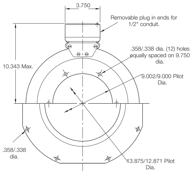
Magnet View
