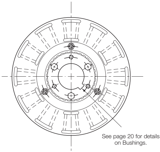
Armature View
