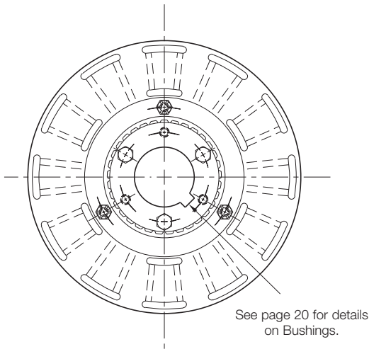
Armature View
