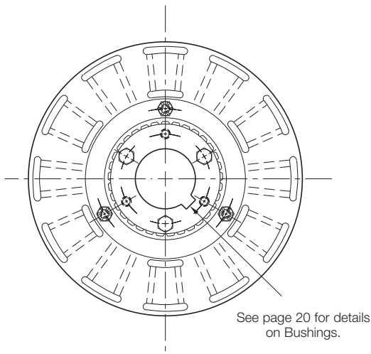
Armature View
