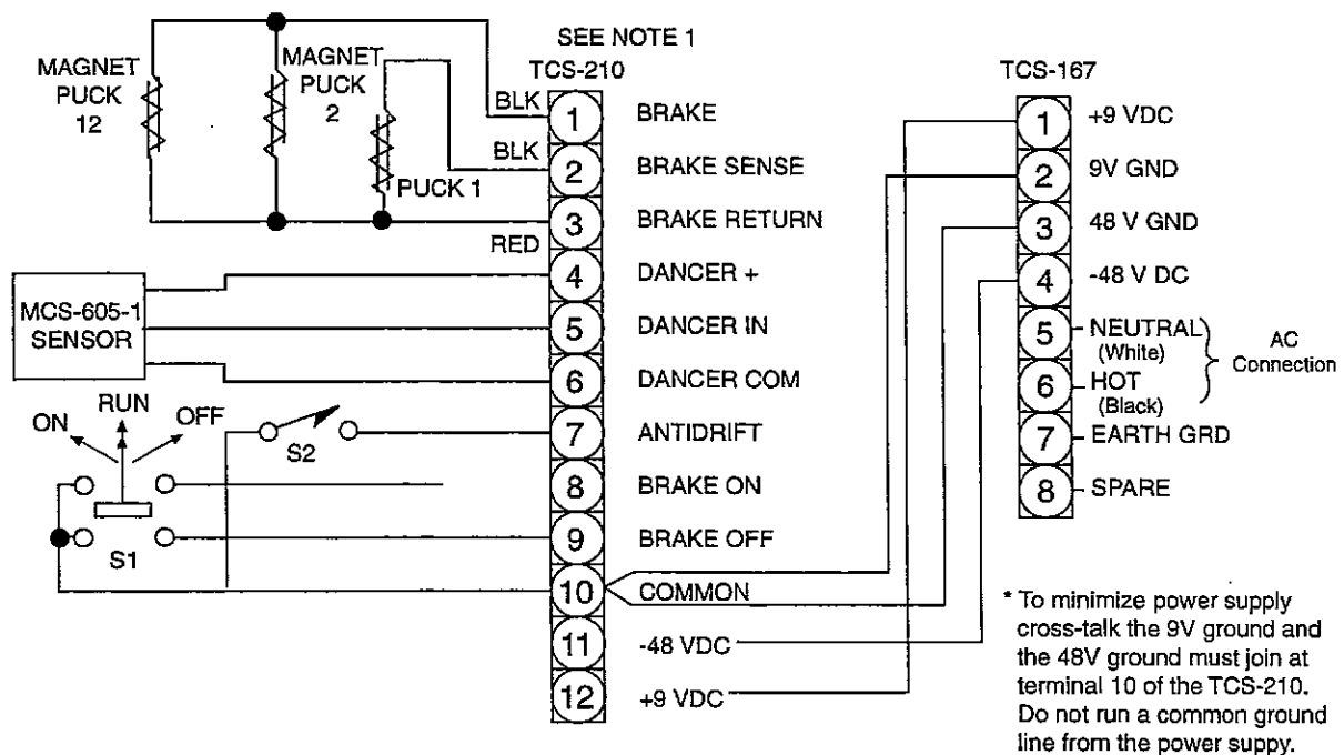
Figure 8 TCS-210 Wiring
