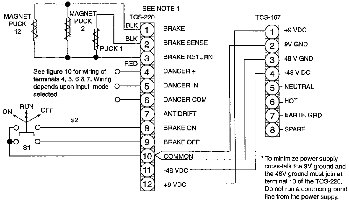
Figure 9 TCS-220 Wiring
