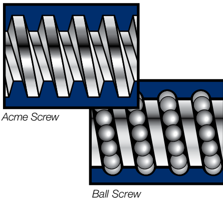
Ball Screw
