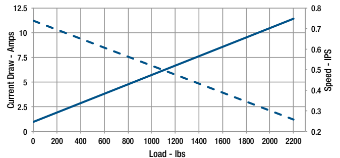
K2XG20-24VDC
