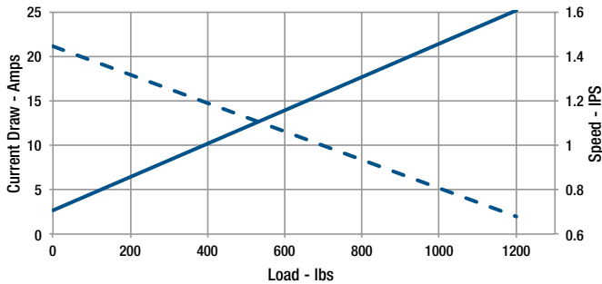
K2XG10-12VDC
