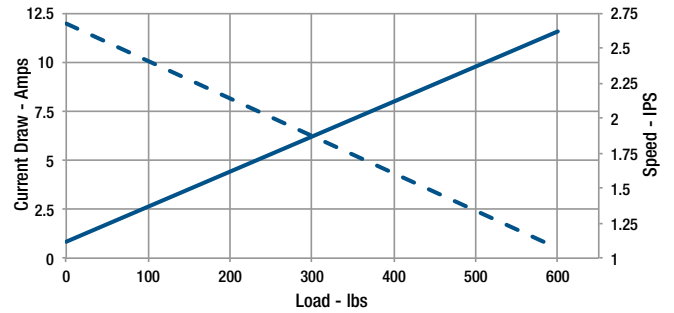
K2XG05-24VDC
