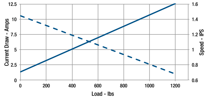
K2XG10-24VDC
