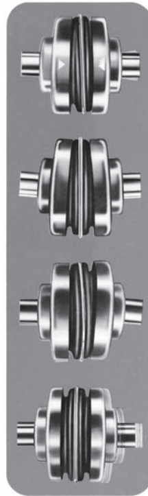
Four basic conditions of shaft misalignment or movement that determine selection of the correct coupling.
