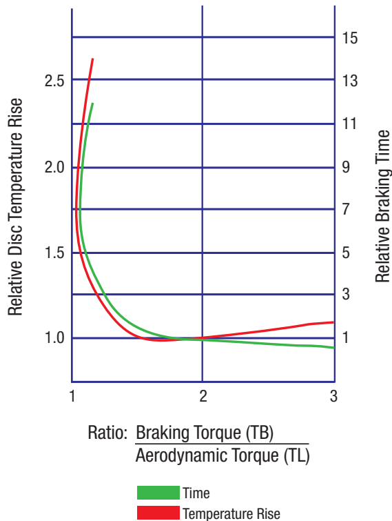
Fig. 1: The ratio of braking torque to aerodynamic torque provides one guide for selecting brakes
