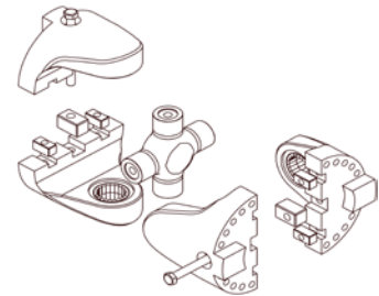
Fig. 6 — Split yoke.
