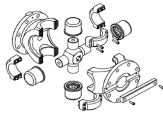
Fig. 7 — Split-bearing eye.
