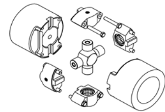
Fig. 8 — Block type.
