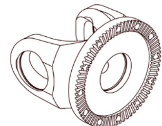
Fig. 10 — Radial face spline.
