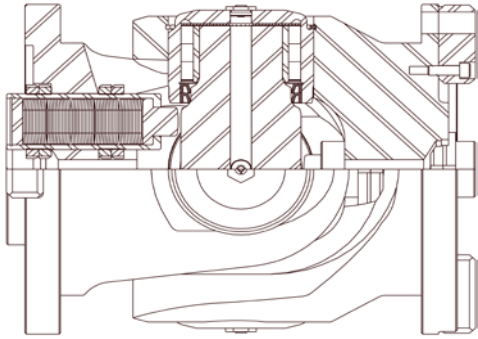
Fig. 12 — Spring angle limiter.
