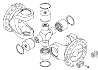
Fig. 5 — Closed-eye (1-piece) yoke.
