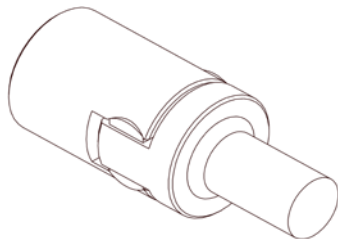
Fig. 3 — Slipper coupling.
