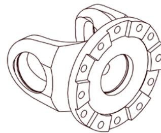
Fig. 9 — Integral face pads.
