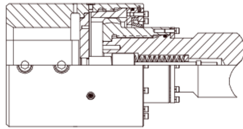
Fig. 4 — Mill gear spindle.
