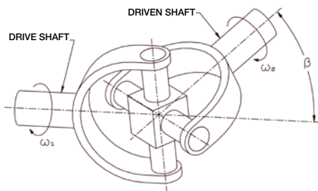
Fig. 1 — Cardan universal joint.
