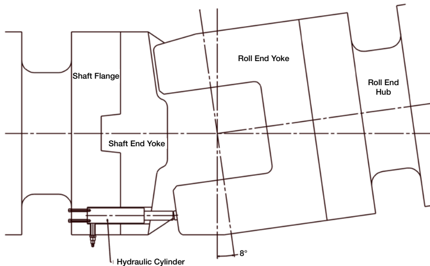
Fig. 14 – Hydraulic angle limiter.
