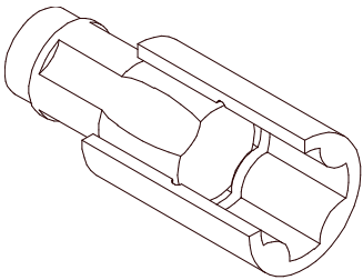
Fig. 2 — Wobbler coupling.
