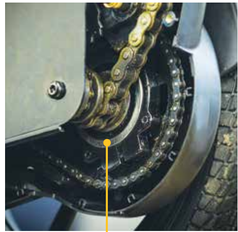
The drive wheel rotates in one direction only, so a freewheel (clutch) is needed to connect the transmission and the drive wheel – just as on a bicycle.
