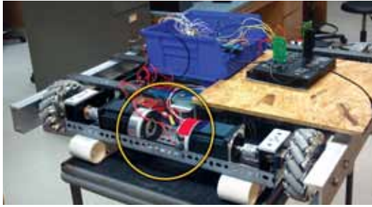
Warner Electric ERS-42 electrically-released, spring-set brakes (shown mounted to stepper motors) are widely used in personal mobility devices.
