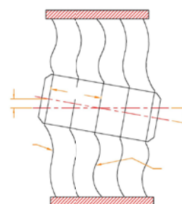
Thin Convoluted Diaphragm
