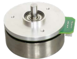
Flat motors offer high torque in compact packages—ideal for wrist and arm integration in humanoid robots.
