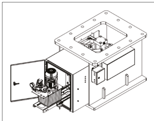
RRC-HS-TF Top Flange model with Local HPU and pullout tray
