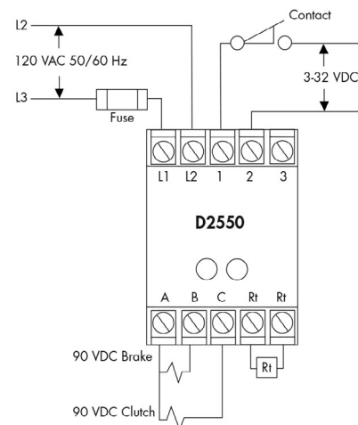
Wiring example for logic input 3-32 VDC
